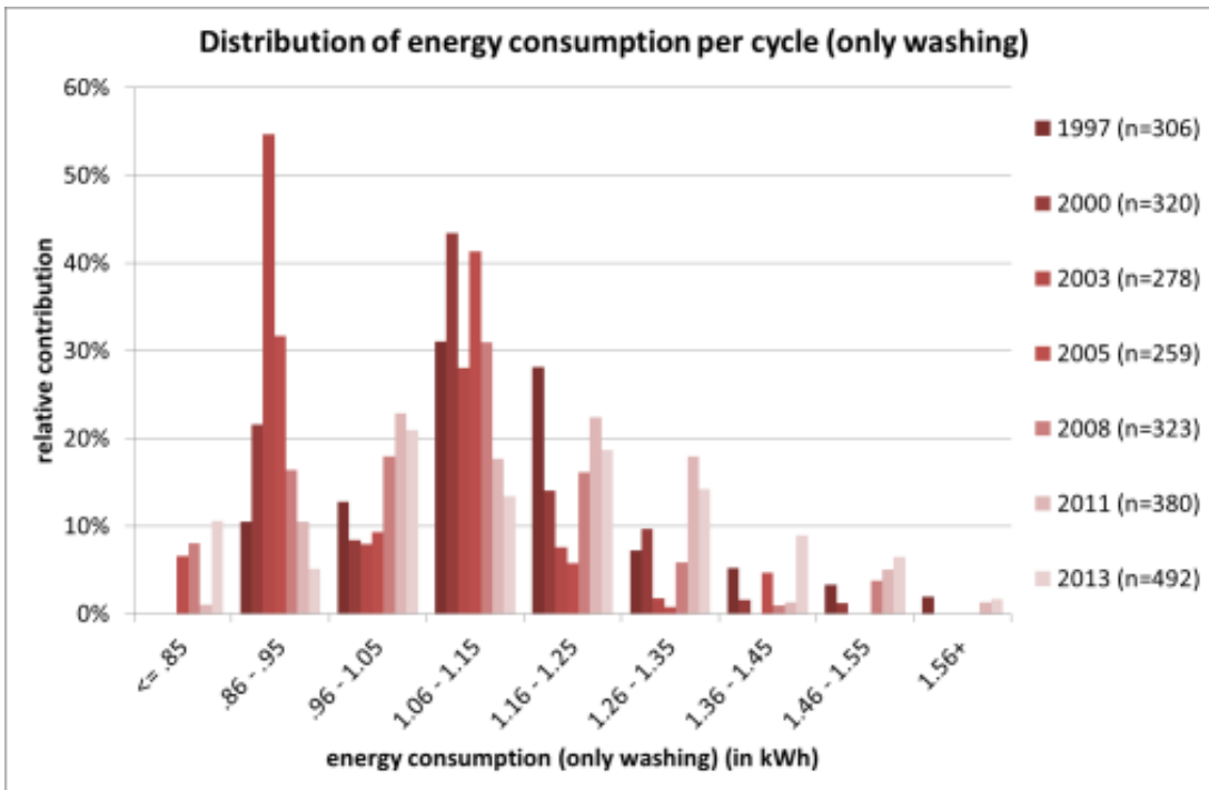
Figure 2.48: Distribution of specific energy consumption for wash cycle of washer-dryer models (CECED 2014)
